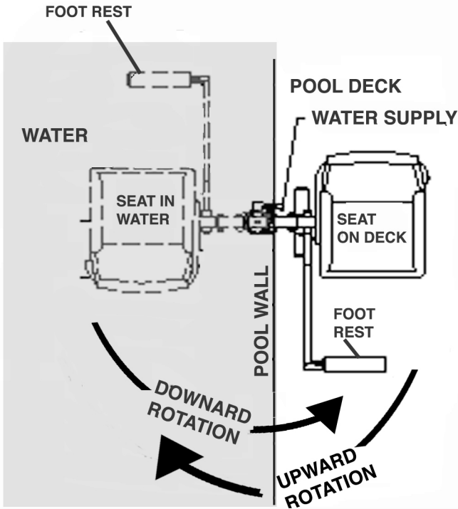
AERIAL VIEW MODEL IGAT-180 STANDARD ROTATION
