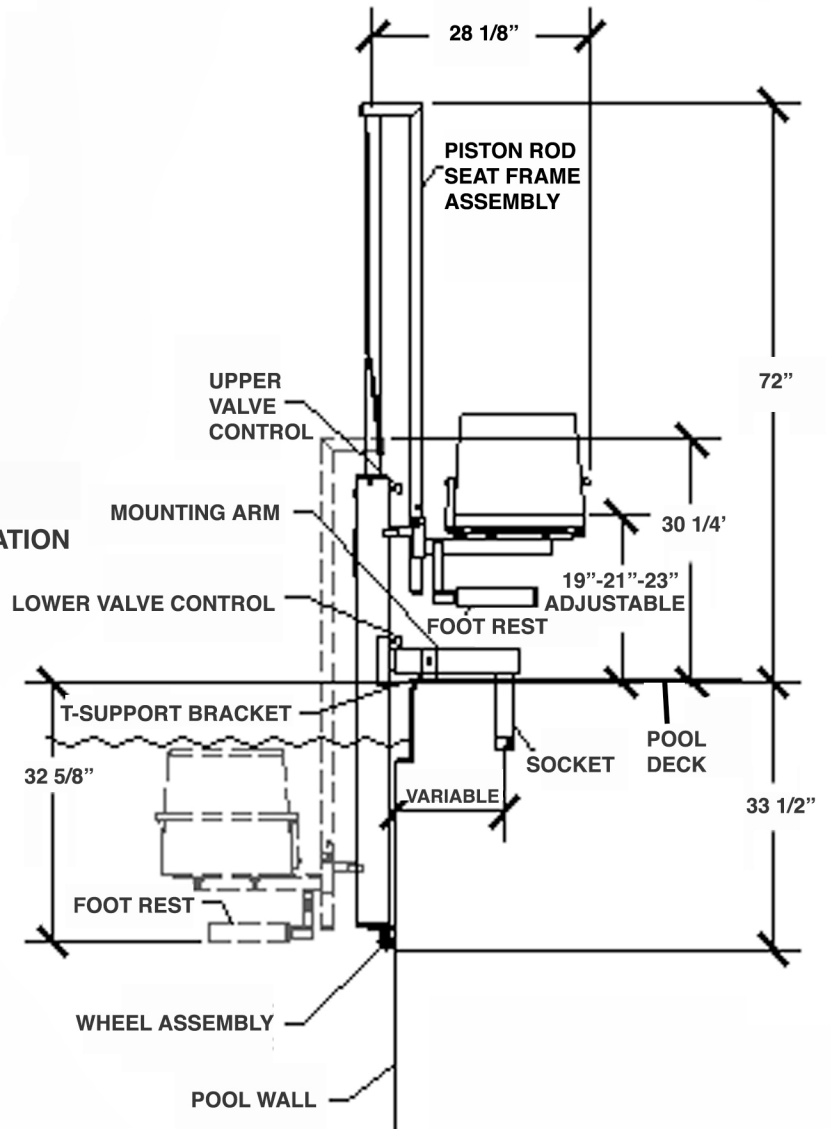
SIDE VIEW MODEL IGAT-180 STANDARD ROTATION
