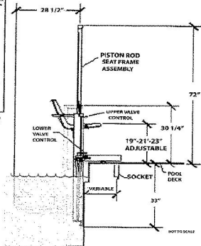
POOL LIFT MODEL IGAT-90 SIDE VIEW
