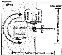
POOL LIFT MODEL IGAT-90 AERIAL VIEW
