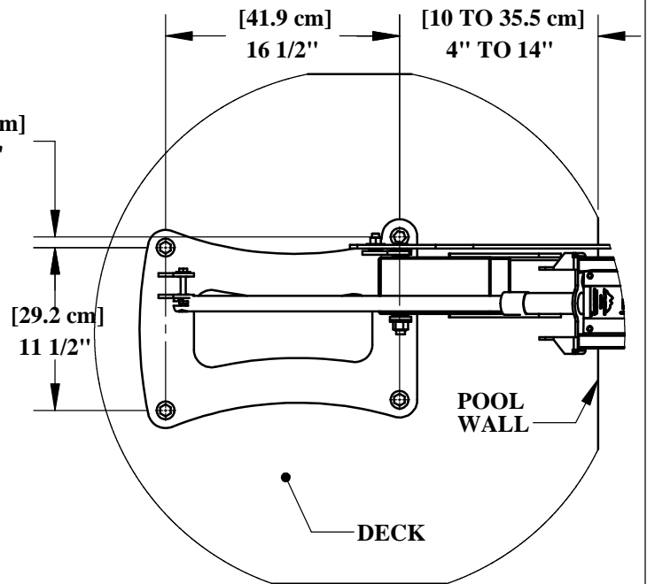
DETAIL A SCALE 1 : 12
