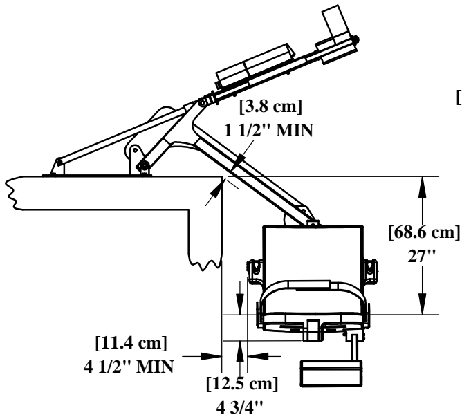
LIFT SHOWN IN FULLY LOWERED POSITION
